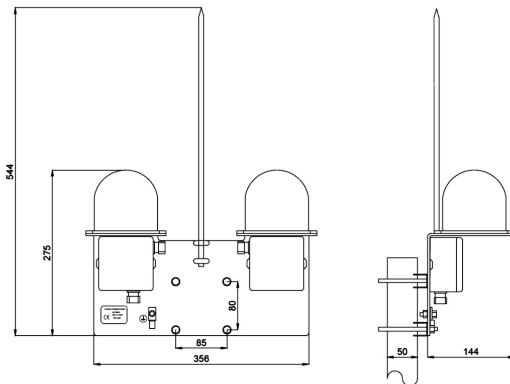
Total dimensions
